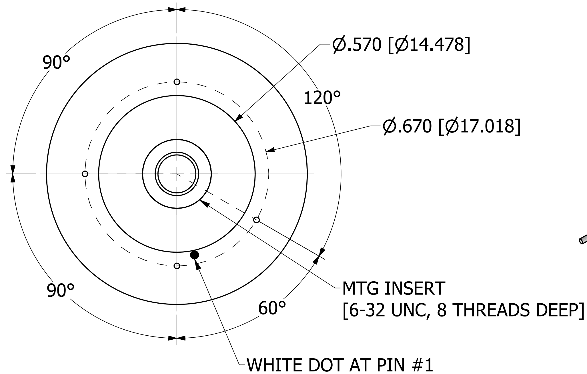
BOTTOM VIEW
